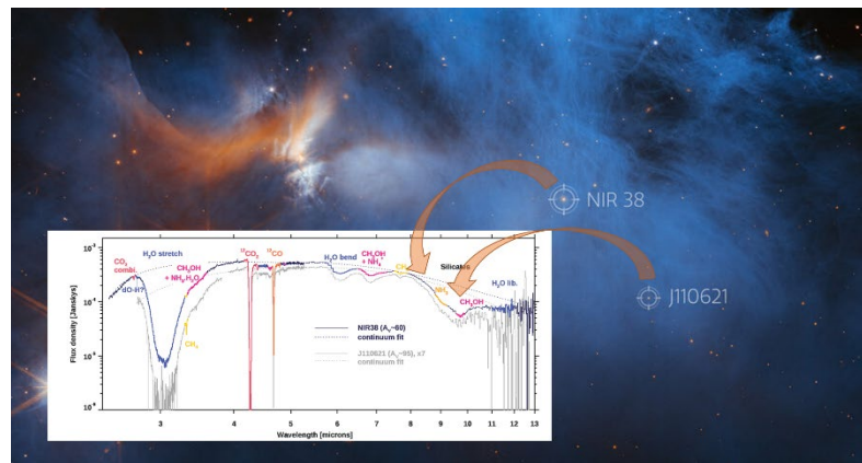
Figure 1: The Chameleon molecular cloud. JWST spectra reveal the composition of interstellar ices in the darkest and densest regions of an interstellar cloud ever measured. The spectra show evidence of several ices and hint at the presence of complex organic molecules.
