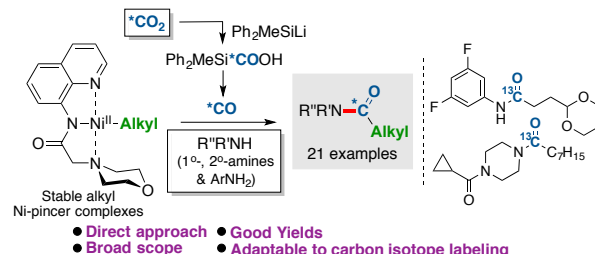
Figure 2: An approach to the carbon isotope-labeling of aliphatic carboxamides exploiting carbon dioxide.
